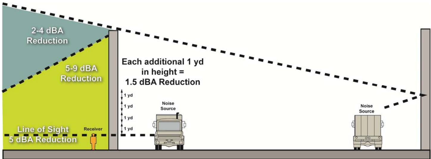
Figure 2.7 Sound barrier noise reduction
